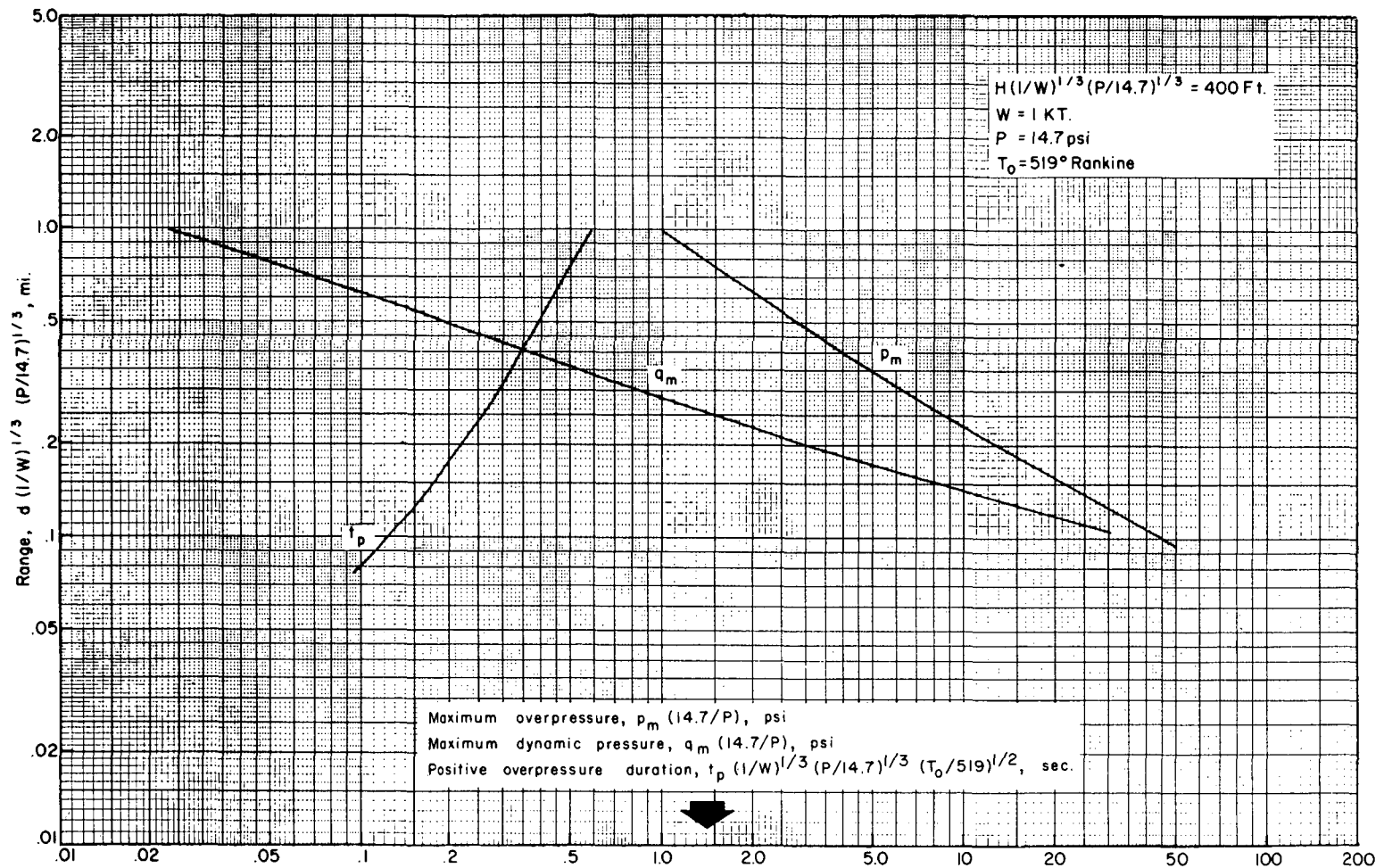
Fig. 2.5—Scaled blast parameters for a scaled height of burst of 400 ft as a function of scaled range. These are plots of Eqs. 2.36, 2.38, and 2.40 given in Table 2.5.
